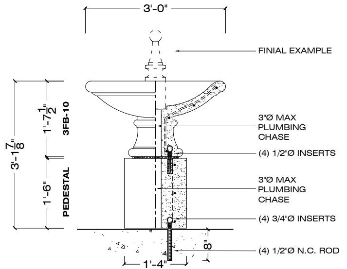
ELEVATION SECTION
