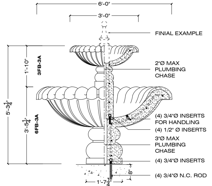
ELEVATION SECTION
