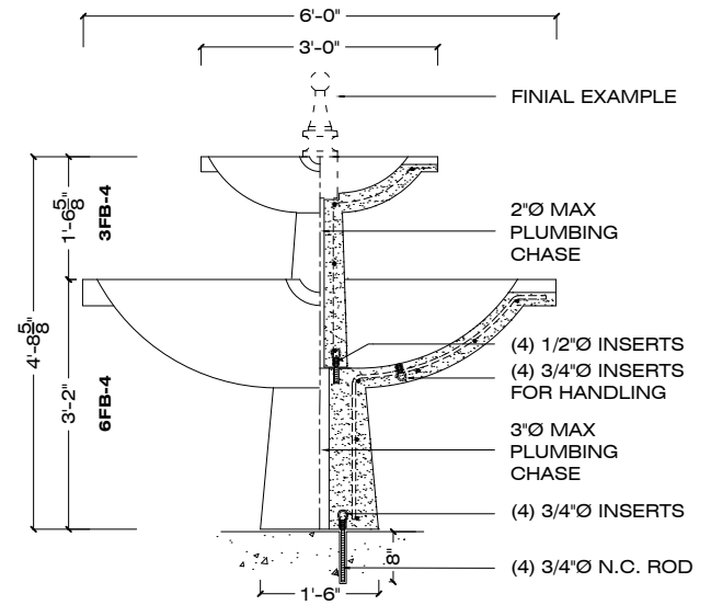
ELEVATION SECTION
