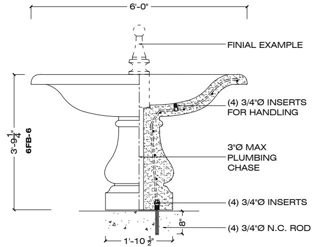
ELEVATION SECTION
