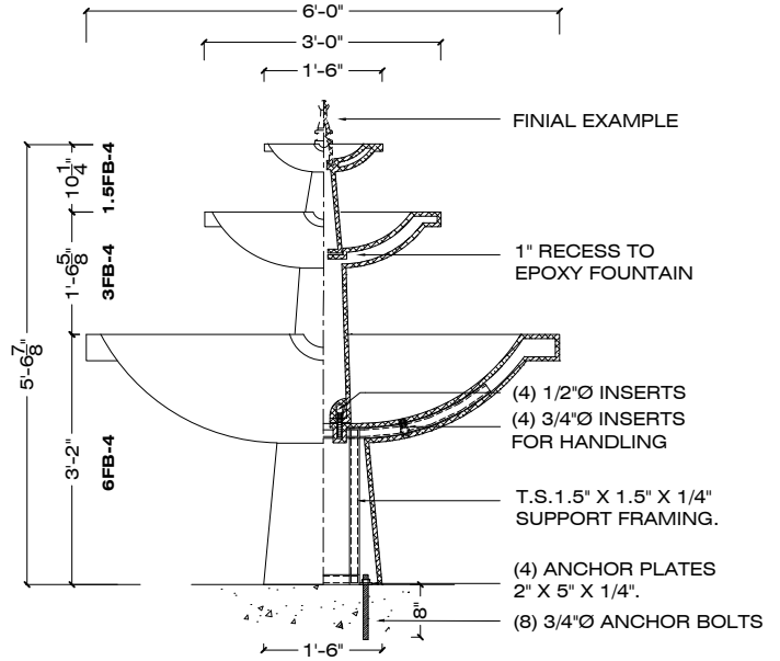
ELEVATION SECTION
