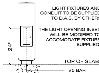
LIGHT BOLLARD MODEL NO - LB-D
