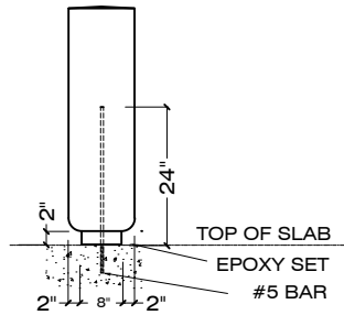
SURFACE MOUNT (B)
