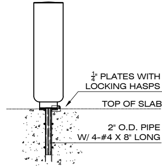
REMOVABLE (C) IN GLASCRETE ONLY
