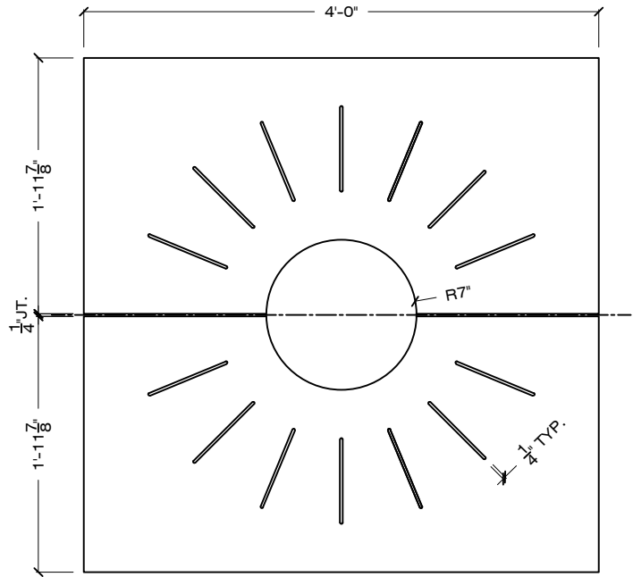
PLAN VIEW
