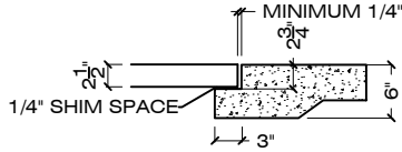
CONCRETE CURB
