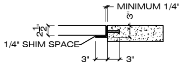
METAL FRAME
