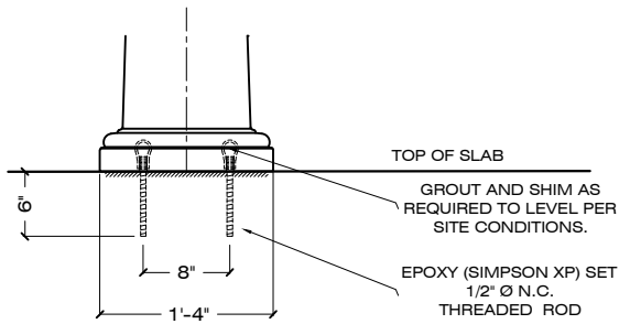
SURFACE MOUNT (B)
