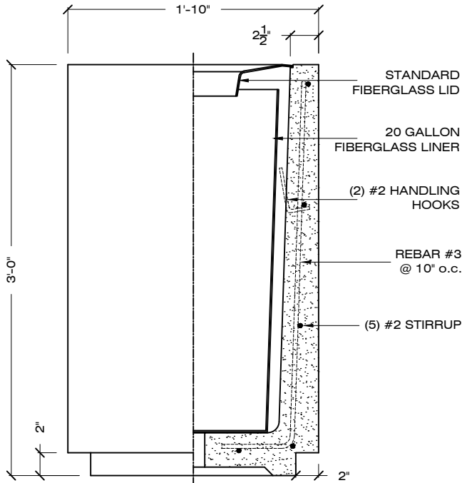
ELEVATION SECTION
