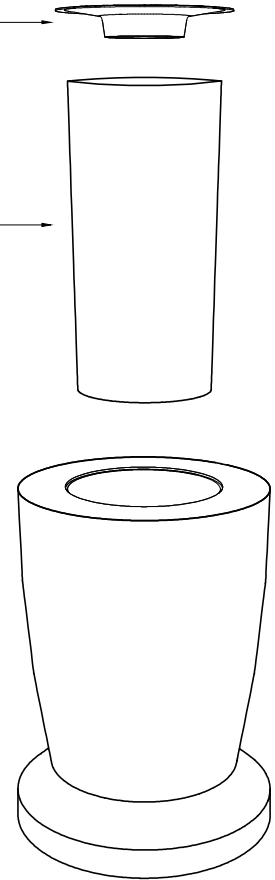
EXPLODED VIEW
