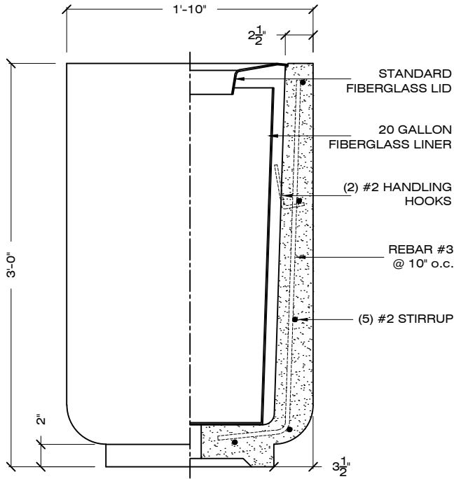
ELEVATION SECTION
