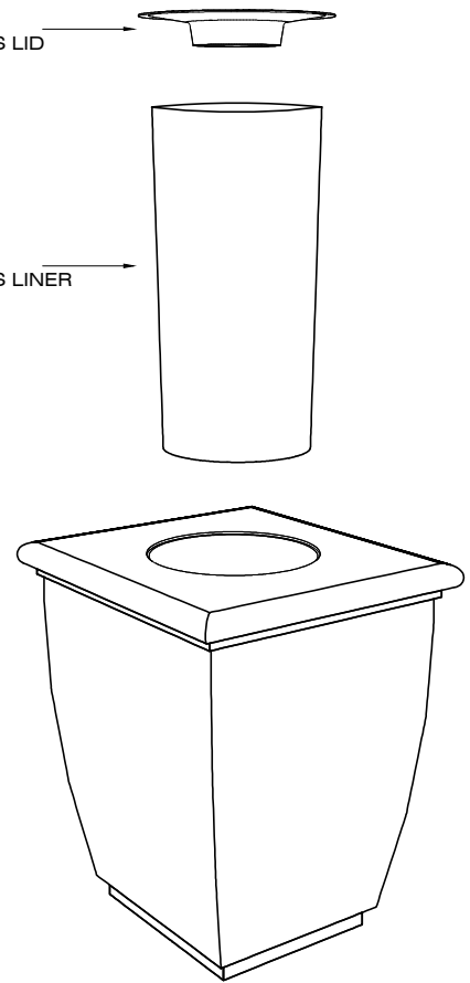
EXPLODED VIEW
