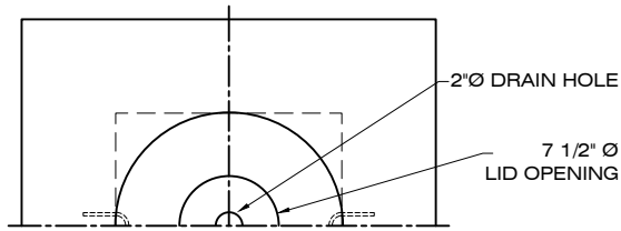
PLAN VIEW
