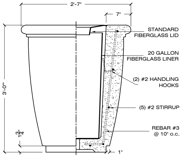
ELEVATION SECTION
