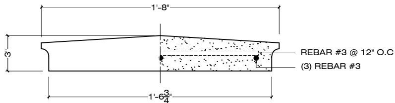
ELEVATION SECTION
