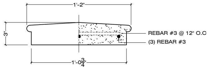
ELEVATION SECTION
