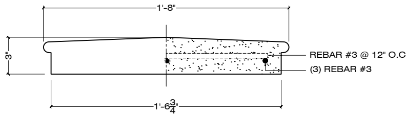
ELEVATION SECTION
