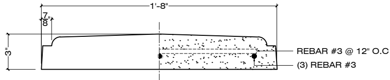
ELEVATION SECTION
