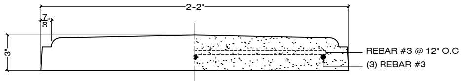
ELEVATION SECTION
