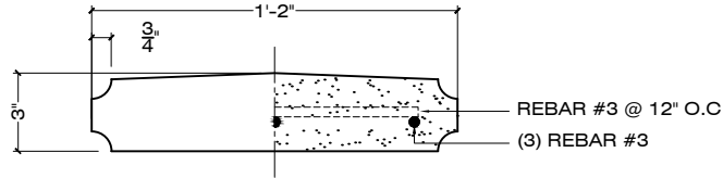
ELEVATION SECTION
