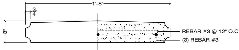
ELEVATION SECTION
