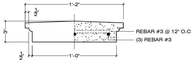
ELEVATION SECTION
