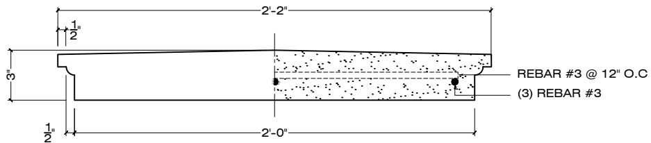
ELEVATION SECTION
