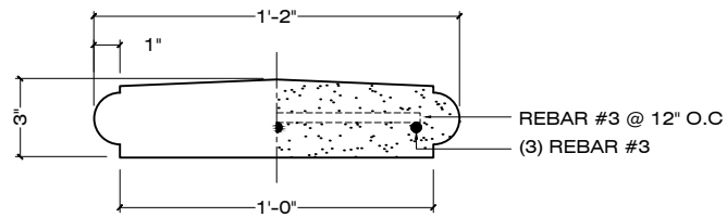
ELEVATION SECTION
