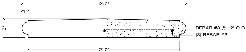
ELEVATION SECTION
