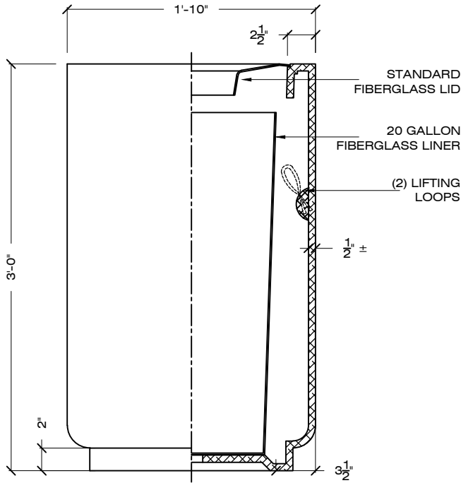
ELEVATION SECTION
