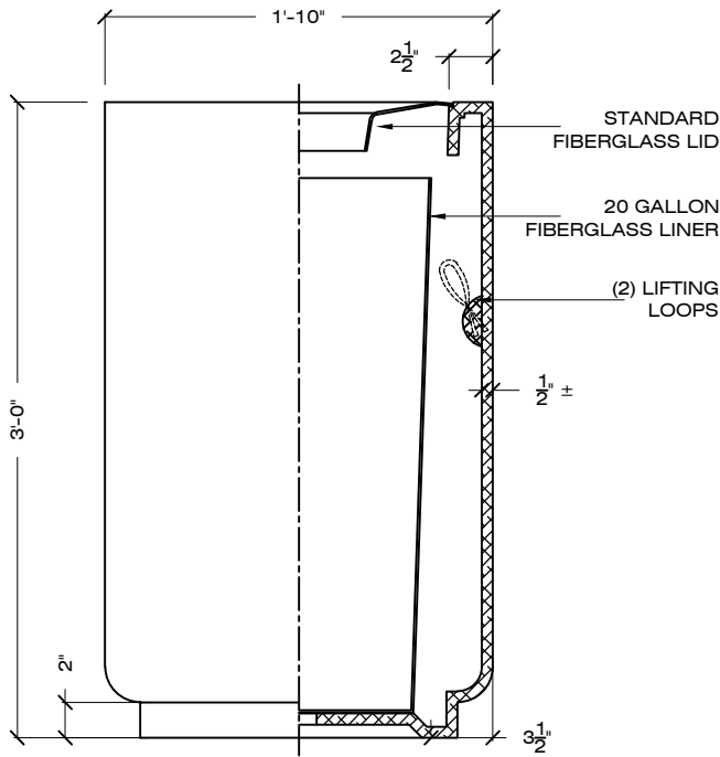
ELEVATION SECTION
