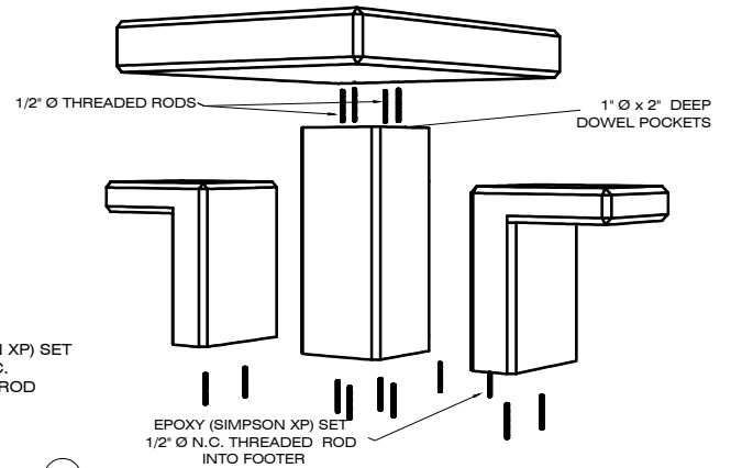
EXPLODED VIEW
