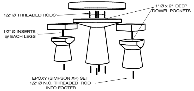
EXPLODED VIEW
