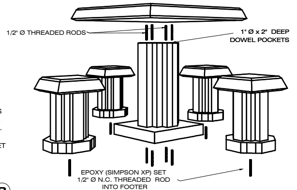
EXPLODED VIEW
