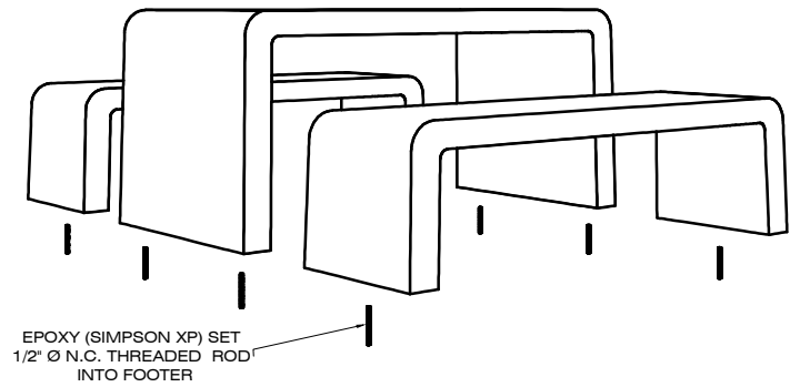
EXPLODED VIEW
