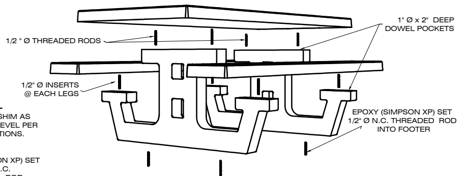
SURFACE MOUNT (B)
