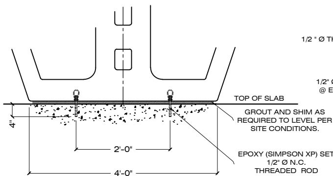
SURFACE MOUNT (B)
