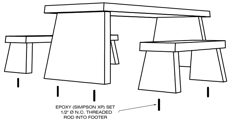
EXPLODED VIEW
