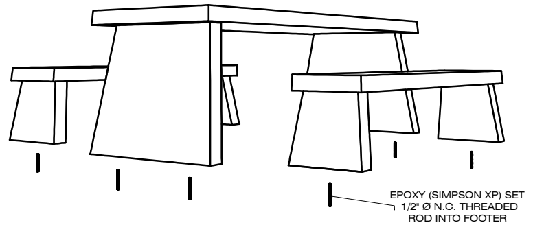
EXPLODED VIEW
