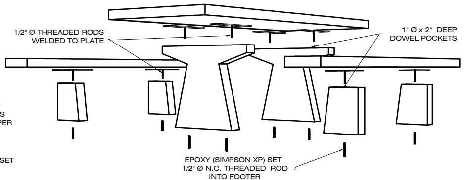
EXPLODED VIEW
