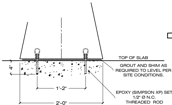
SURFACE MOUNT (B)
