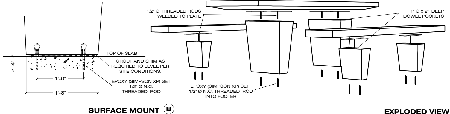
EXPLODED VIEW
