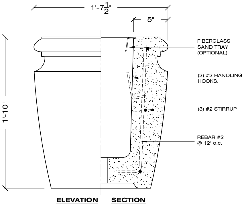
ELEVATION SECTION
