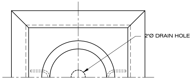
PLAN VIEW
