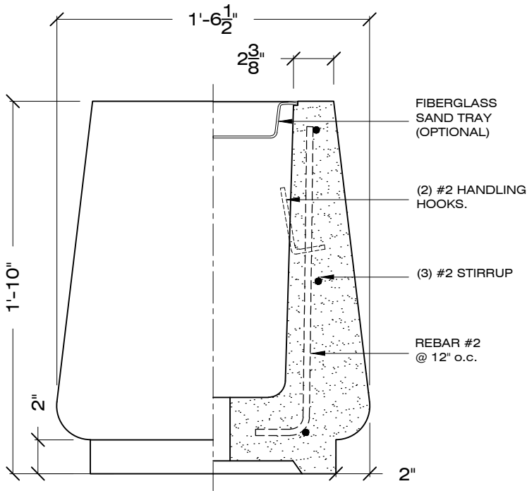
ELEVATION SECTION
