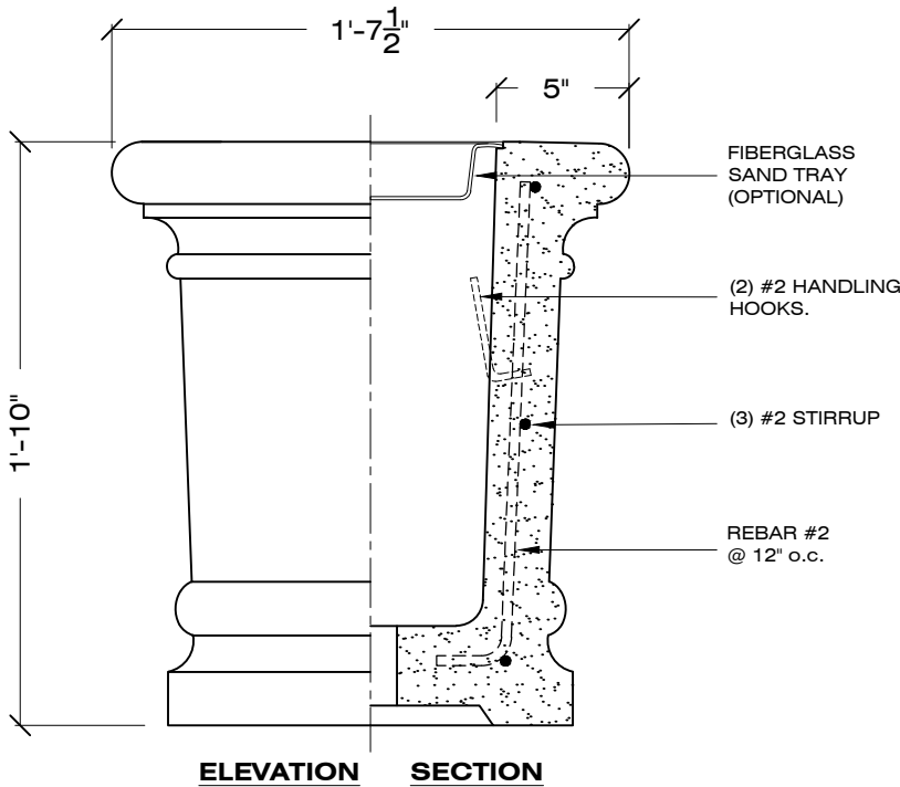
ELEVATION SECTION
