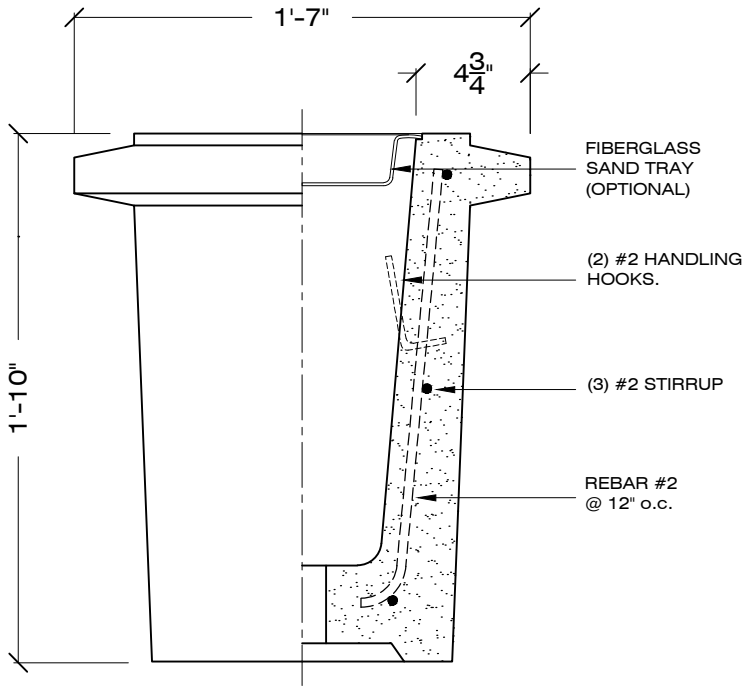
ELEVATION SECTION
