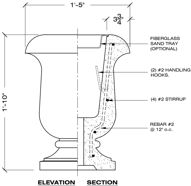
ELEVATION SECTION
