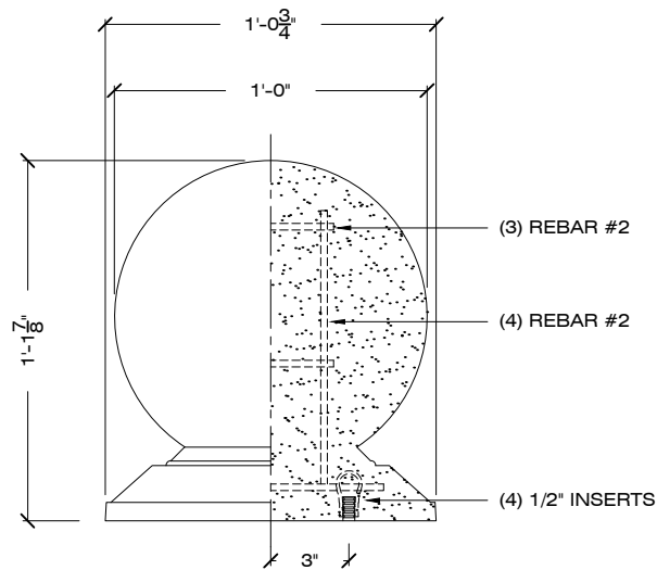
ELEVATION SECTION
