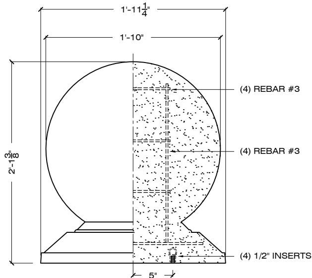
ELEVATION SECTION
