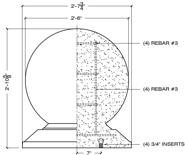
ELEVATION SECTION
