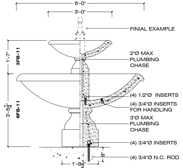
ELEVATION SECTION
