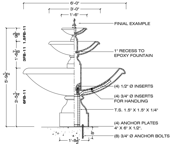
ELEVATION SECTION
