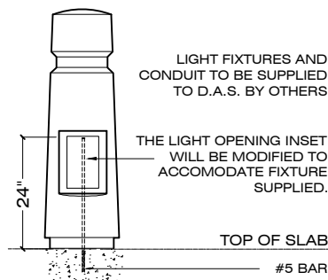
LIGHT BOLLARD MODEL NO - LB-H2
