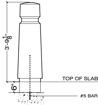
SUBTERRANEAN MOUNT (A)
