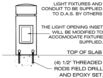
LIGHT BOLLARD MODEL NO - LB-H4
