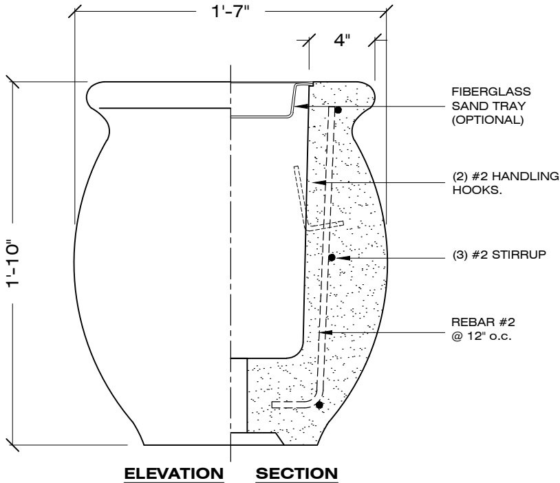
ELEVATION SECTION
