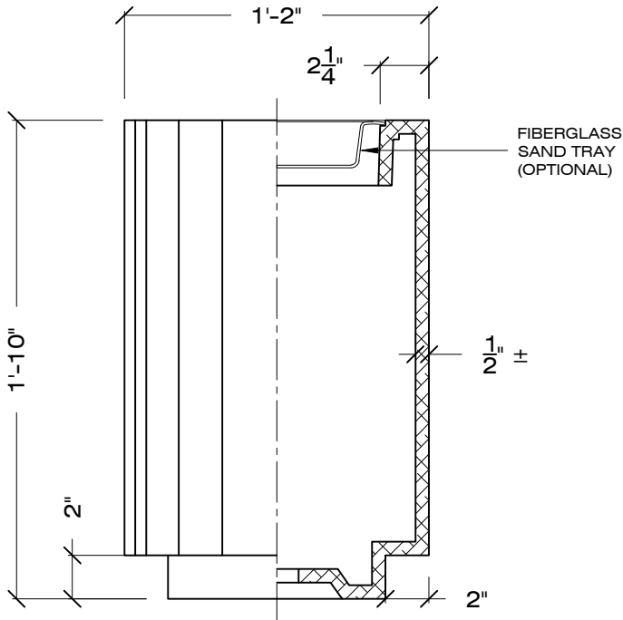
ELEVATION SECTION
